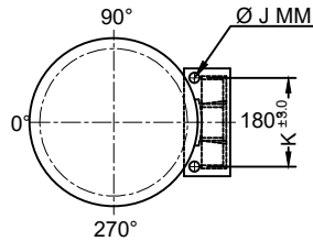
FOUNDATION DETAIL
